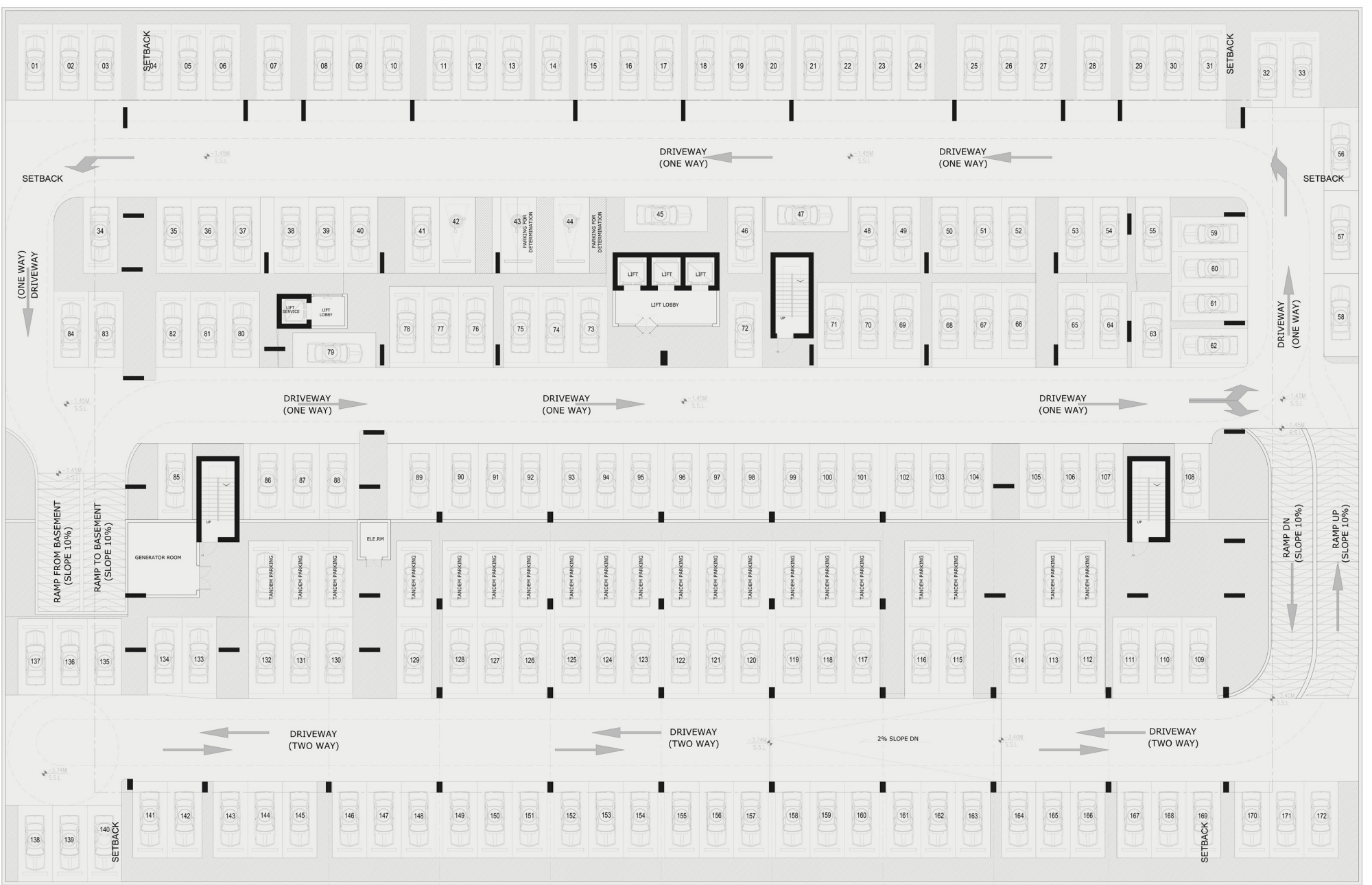
BASEMENT FLOOR PLAN PARKING NUMBER - 170 NO.S
